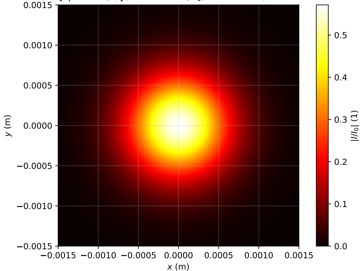
Intensity profile I(x, y, z = 2.309m)/I_0 , Pin=0.3Pcr, artificial time
